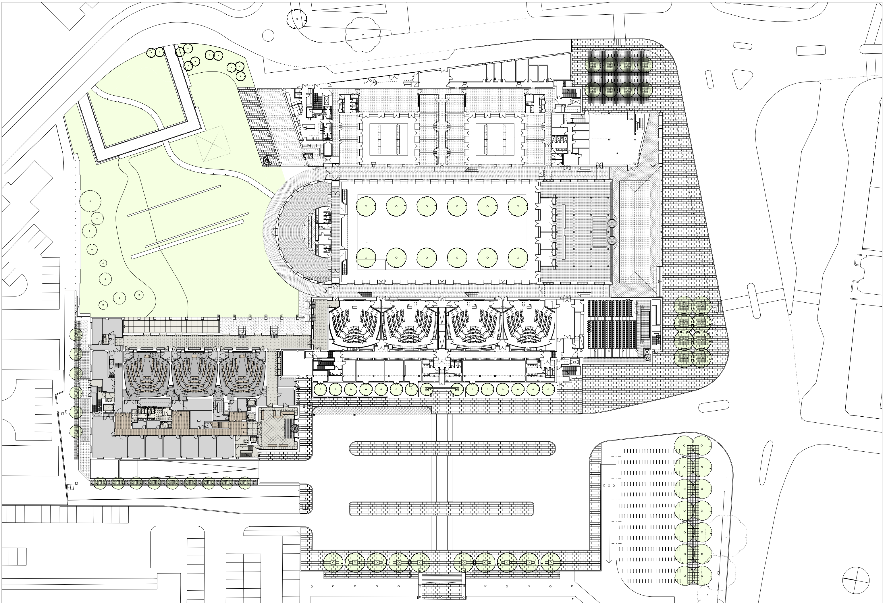
SITE PLAN
